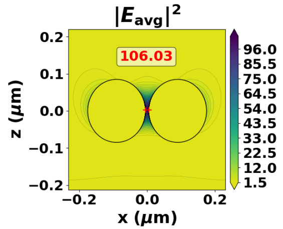
(b) d = 10 \text{ nm} , \lambda = 700 \text{ nm} .
