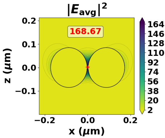
(a) d = 5 \text{ nm} , \lambda = 730 \text{ nm} .
