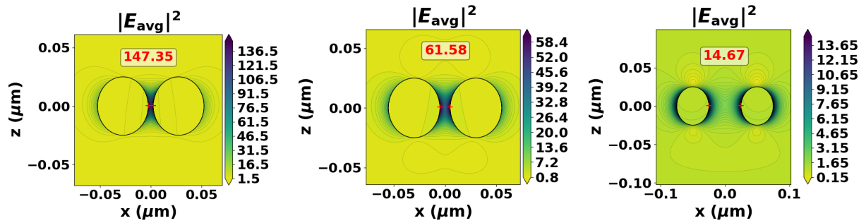
(a) d = 5 \text{ nm} , \lambda = 530 \text{ nm} . Máximo: 147.35 |E_0|^2 . (b) d = 10 \text{ nm} , \lambda = 525 \text{ nm} . Máximo: 61.58 |E_0|^2 . (c) d = 50 \text{ nm} , \lambda = 520 \text{ nm} . Máximo: 14.67 |E_0|^2 .
