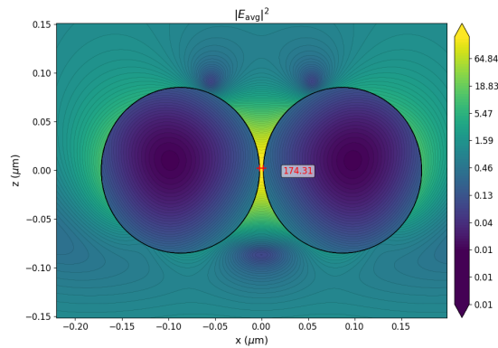
(a) d = 4 \text{ nm} , \lambda = 720 \text{ nm} . Máximo: 174.31 |\mathbf{E}_0|^2 .
