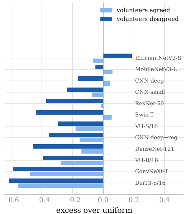
(b) soft-label models, by agreement
