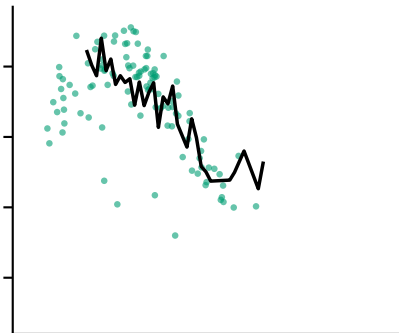
lstm
