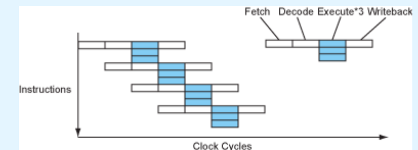
Figure 6 - The instruction flow of a VLIW processor.
