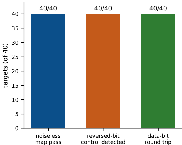
(a) Independent deterministic mapping audit
