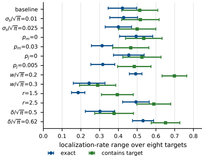
(b) Digitized-GKP one-factor sensitivity
