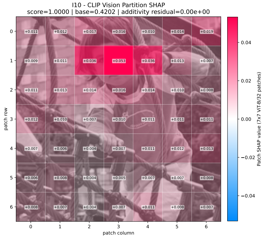
Figure 36: CLIP vision, image I10: 7×7 patch SHAP values over the 224×224 model input.
