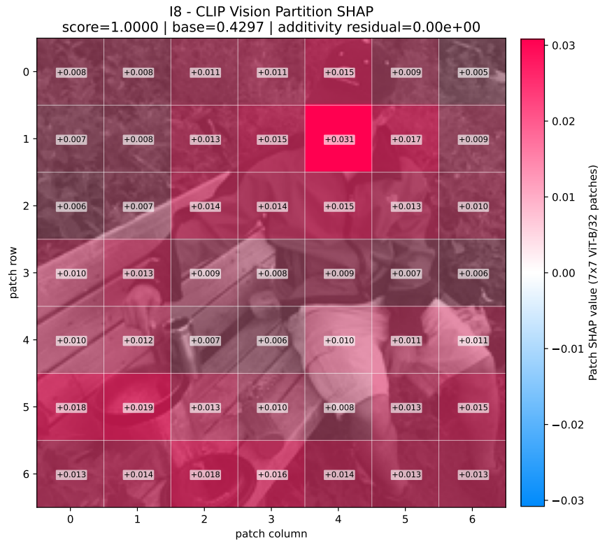
Figure 34: CLIP vision, image I8: 7 \times 7 patch SHAP values over the 224 \times 224 model input.
