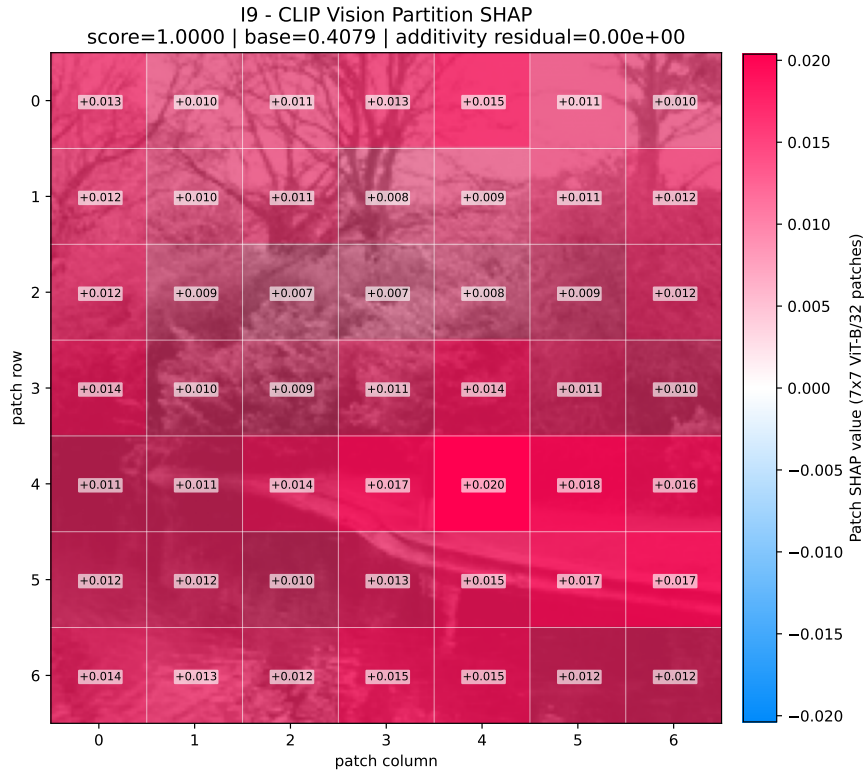
Figure 35: CLIP vision, image I9: 7×7 patch SHAP values over the 224×224 model input.
