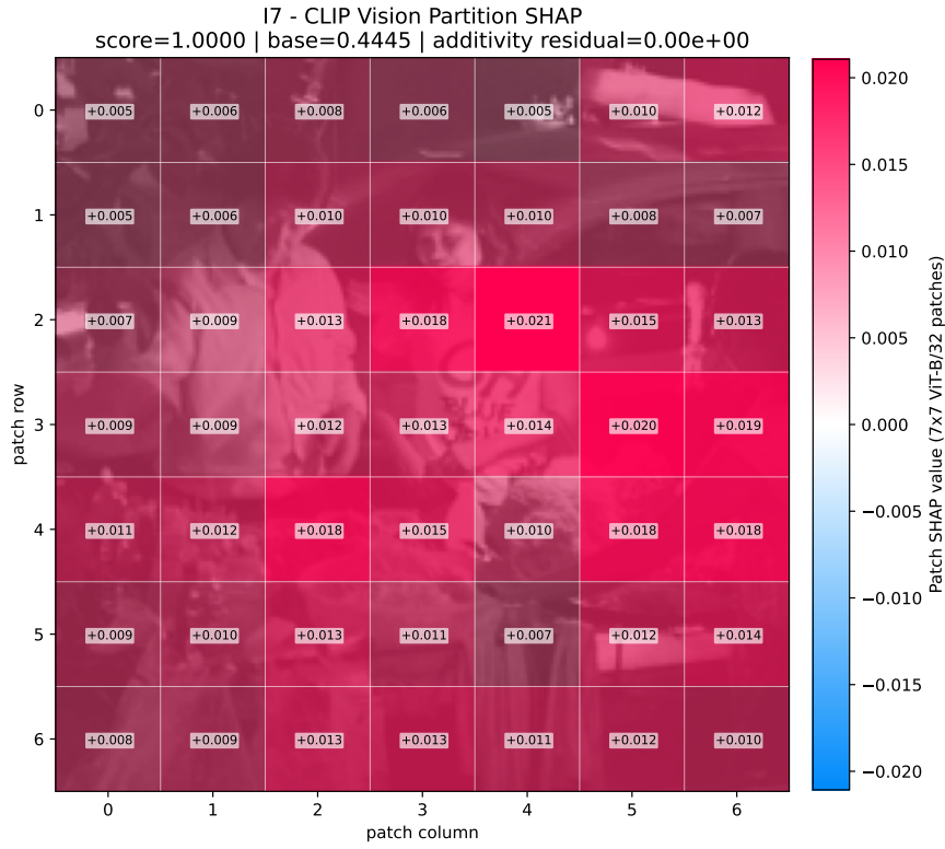
Figure 33: CLIP vision, image I7: 7 \times 7 patch SHAP values over the 224 \times 224 model input.
