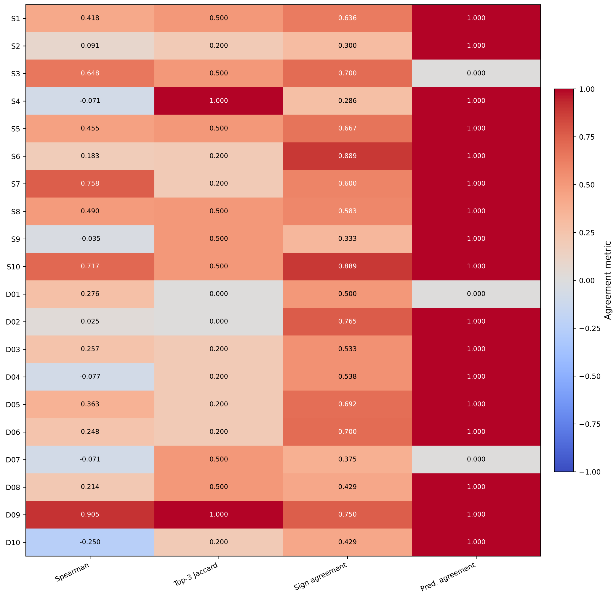
BERT versus CLIP text SHAP ranking comparison
