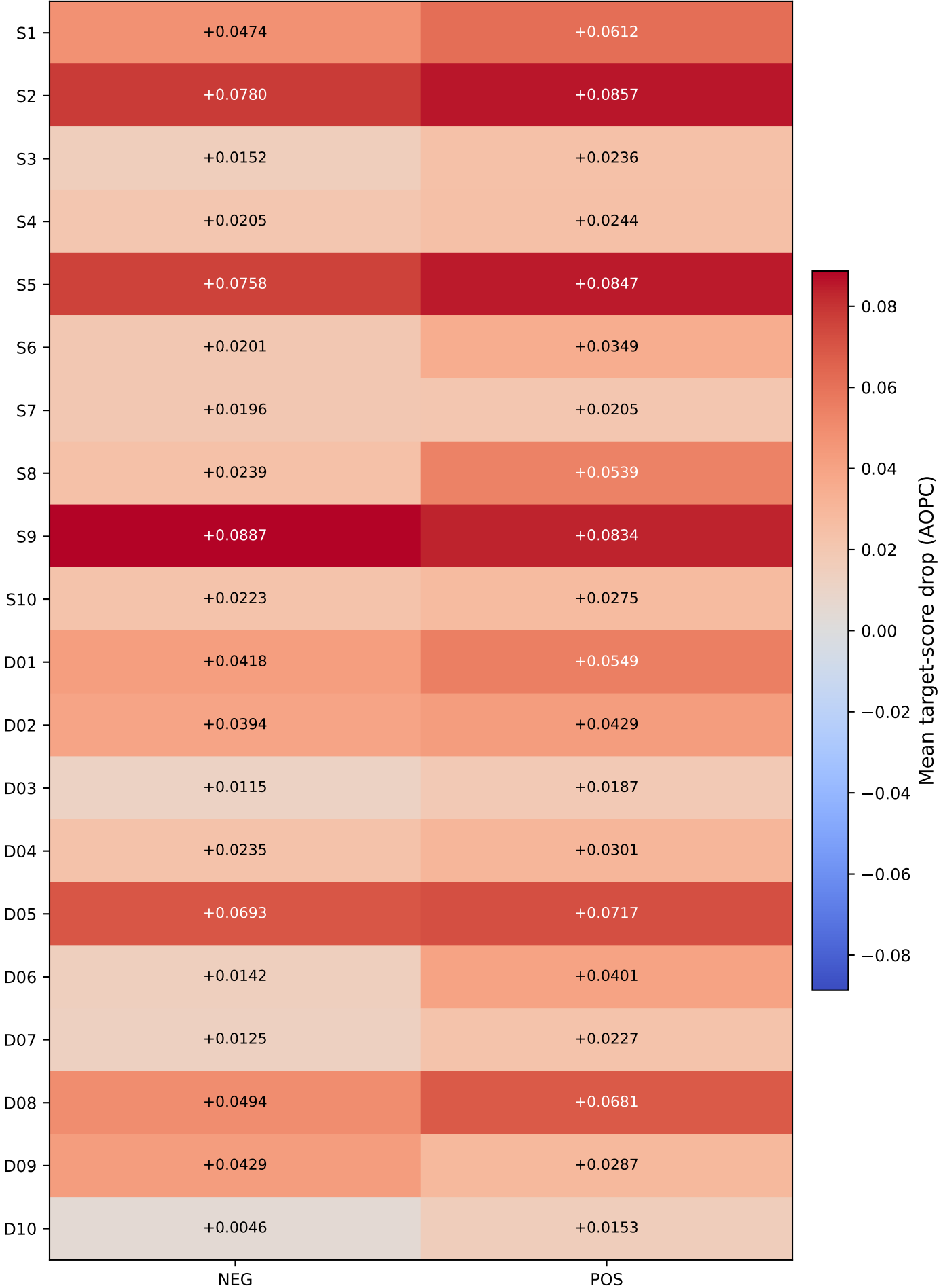
Per-sentence AOPC for SHAP top-k deletion
