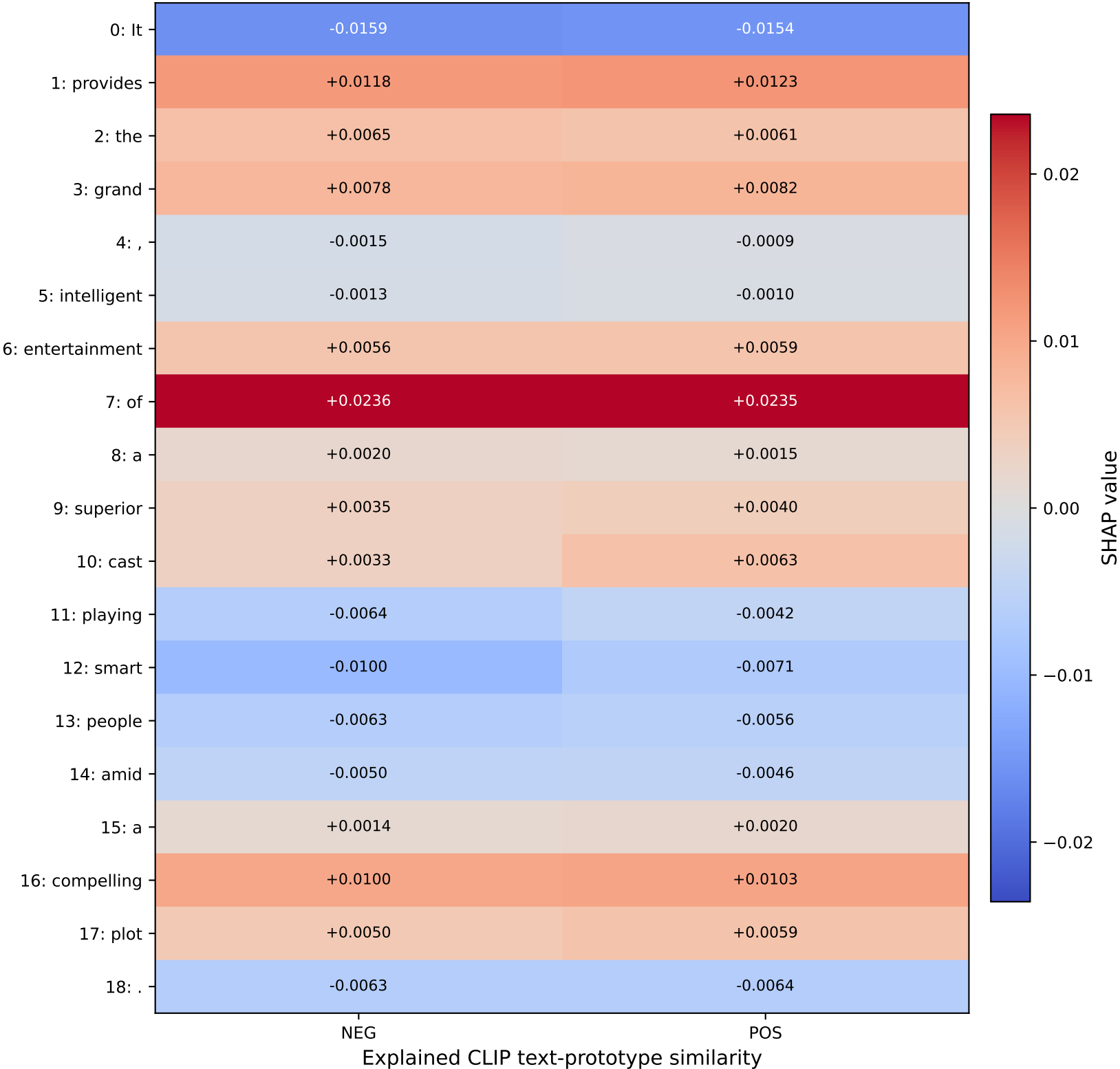
D02: Word-by-class SHAP matrix
