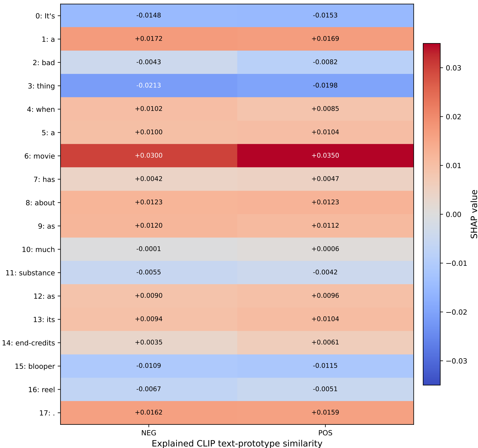
D03: Word-by-class SHAP matrix
