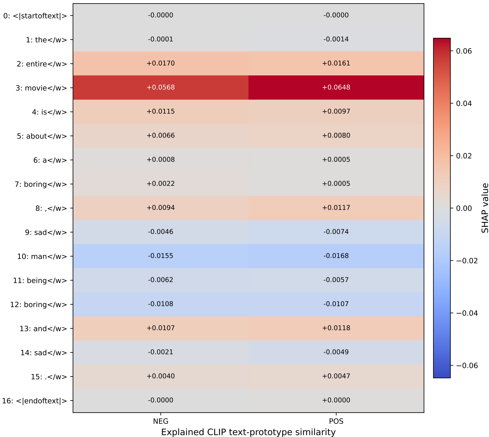
D05: Token-by-class SHAP matrix
