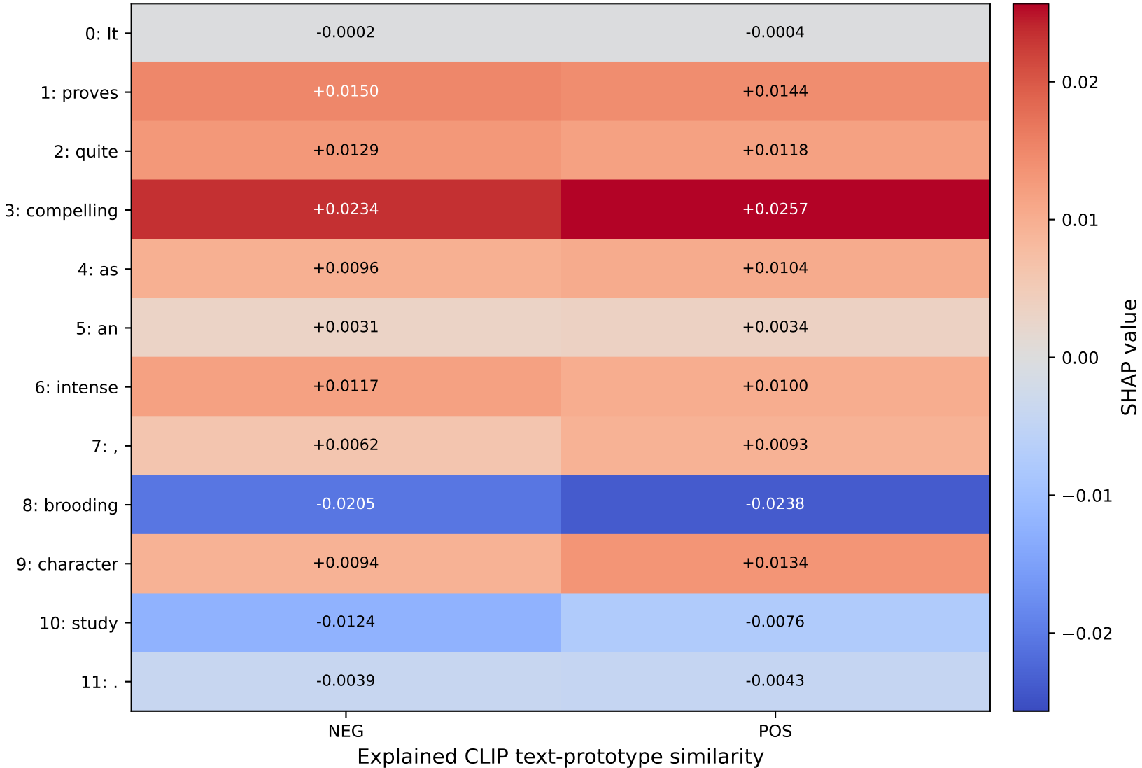
D06: Word-by-class SHAP matrix
