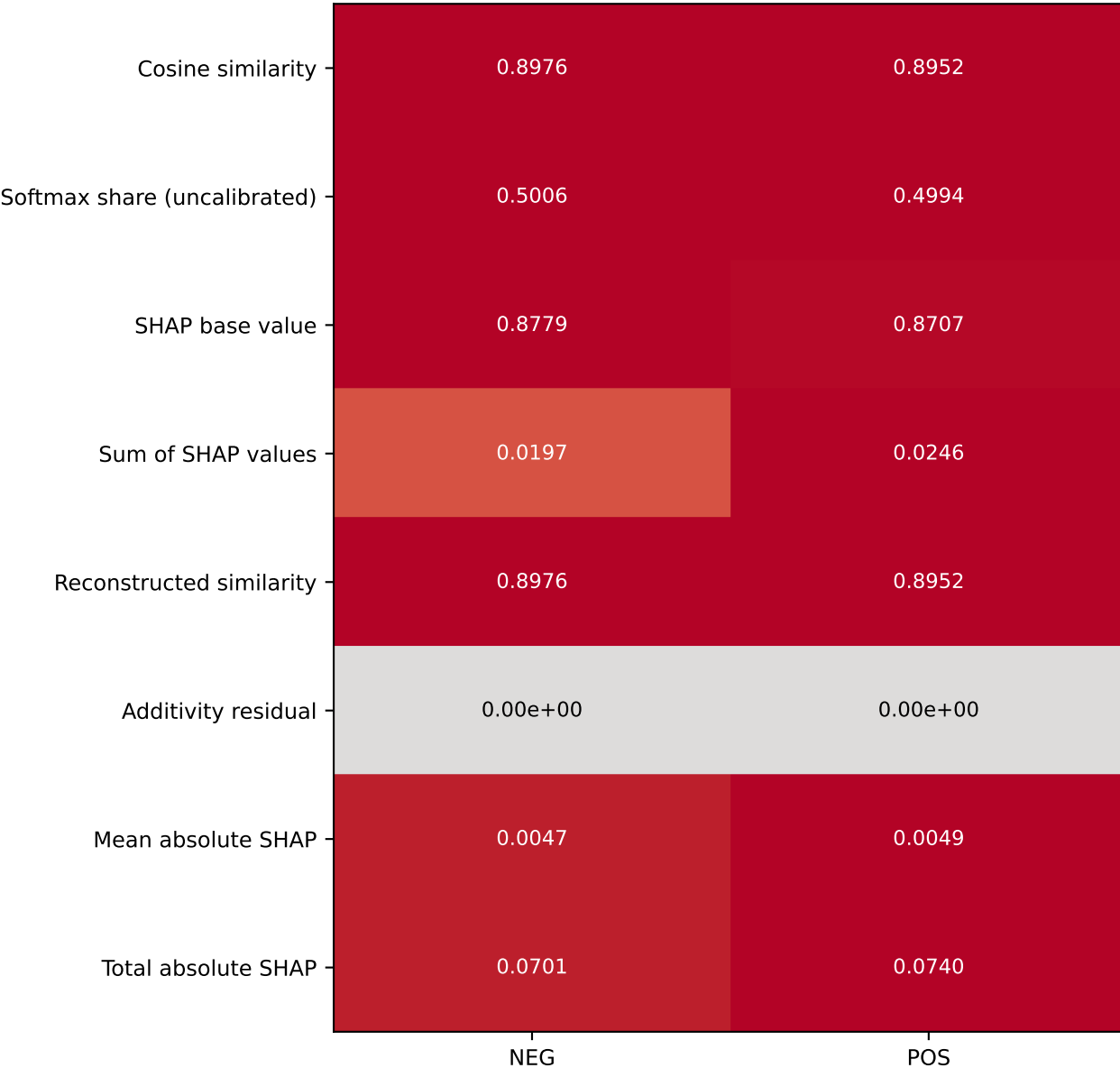
Sentence-summary values
