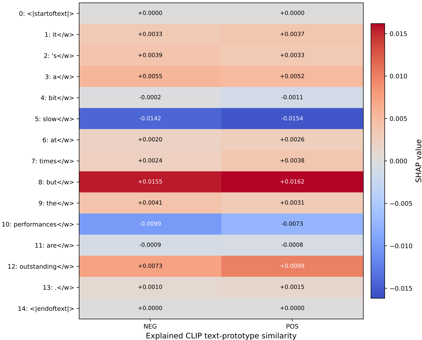
S3: Token-by-class SHAP matrix
