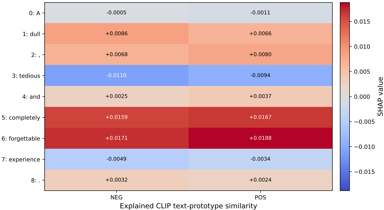
S4: Word-by-class SHAP matrix
