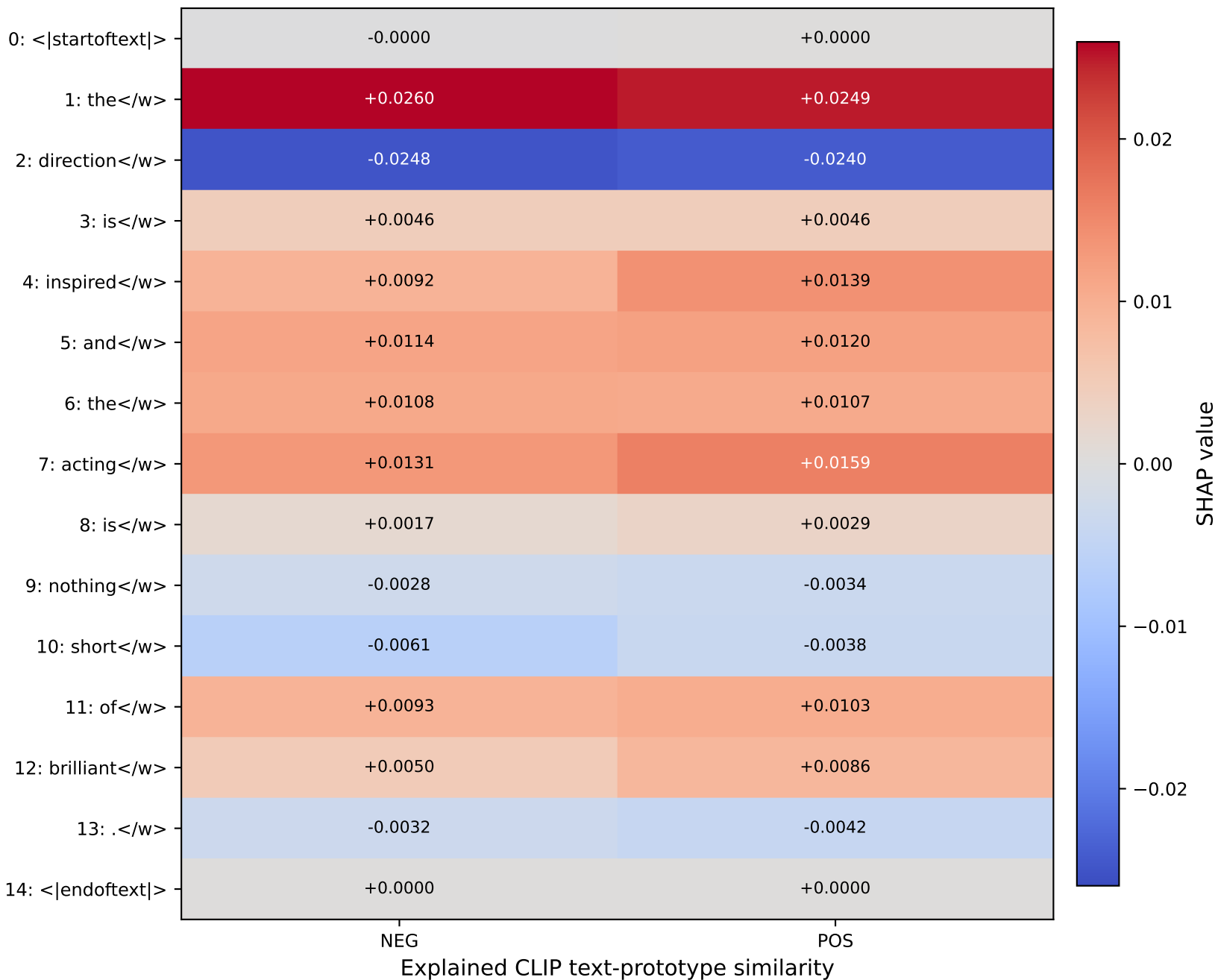
S5: Token-by-class SHAP matrix
