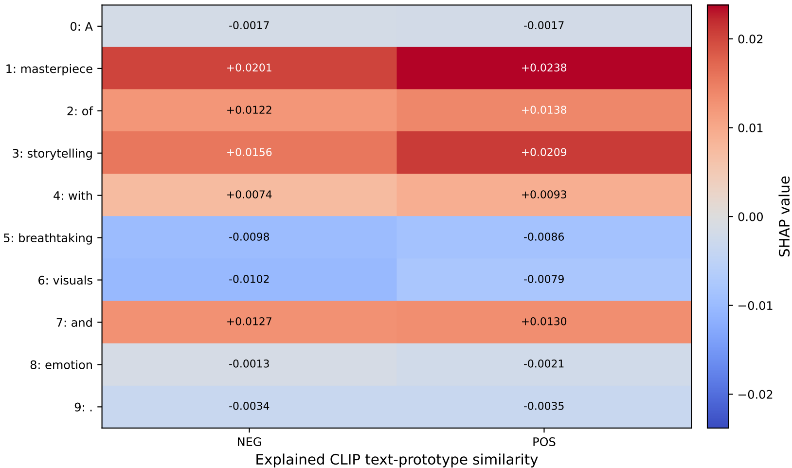
S6: Word-by-class SHAP matrix
