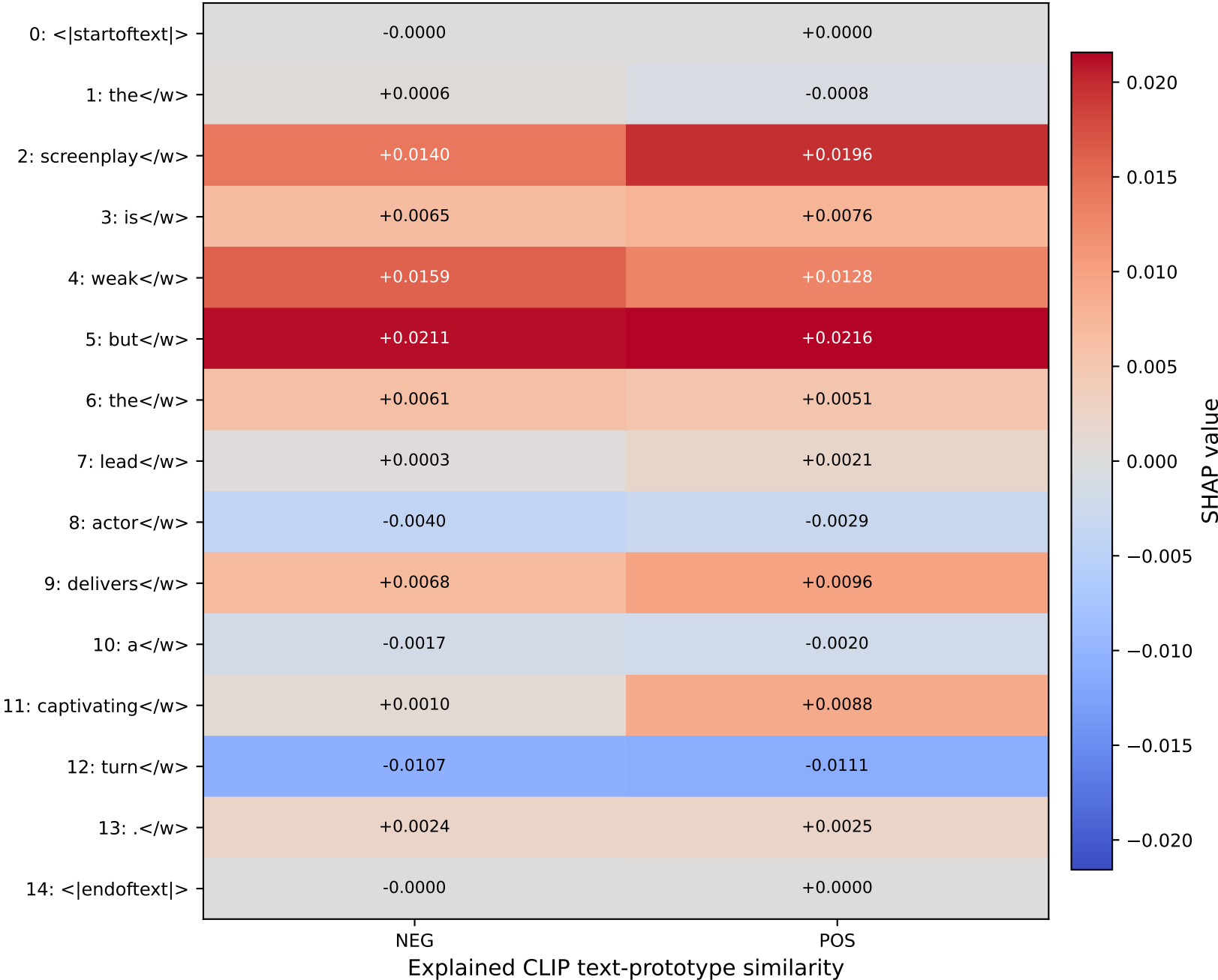
S8: Token-by-class SHAP matrix
