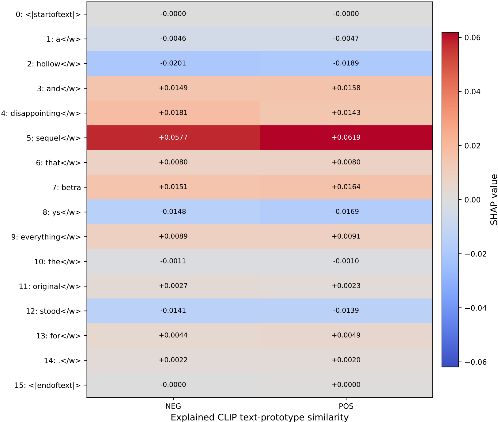
S9: Token-by-class SHAP matrix
