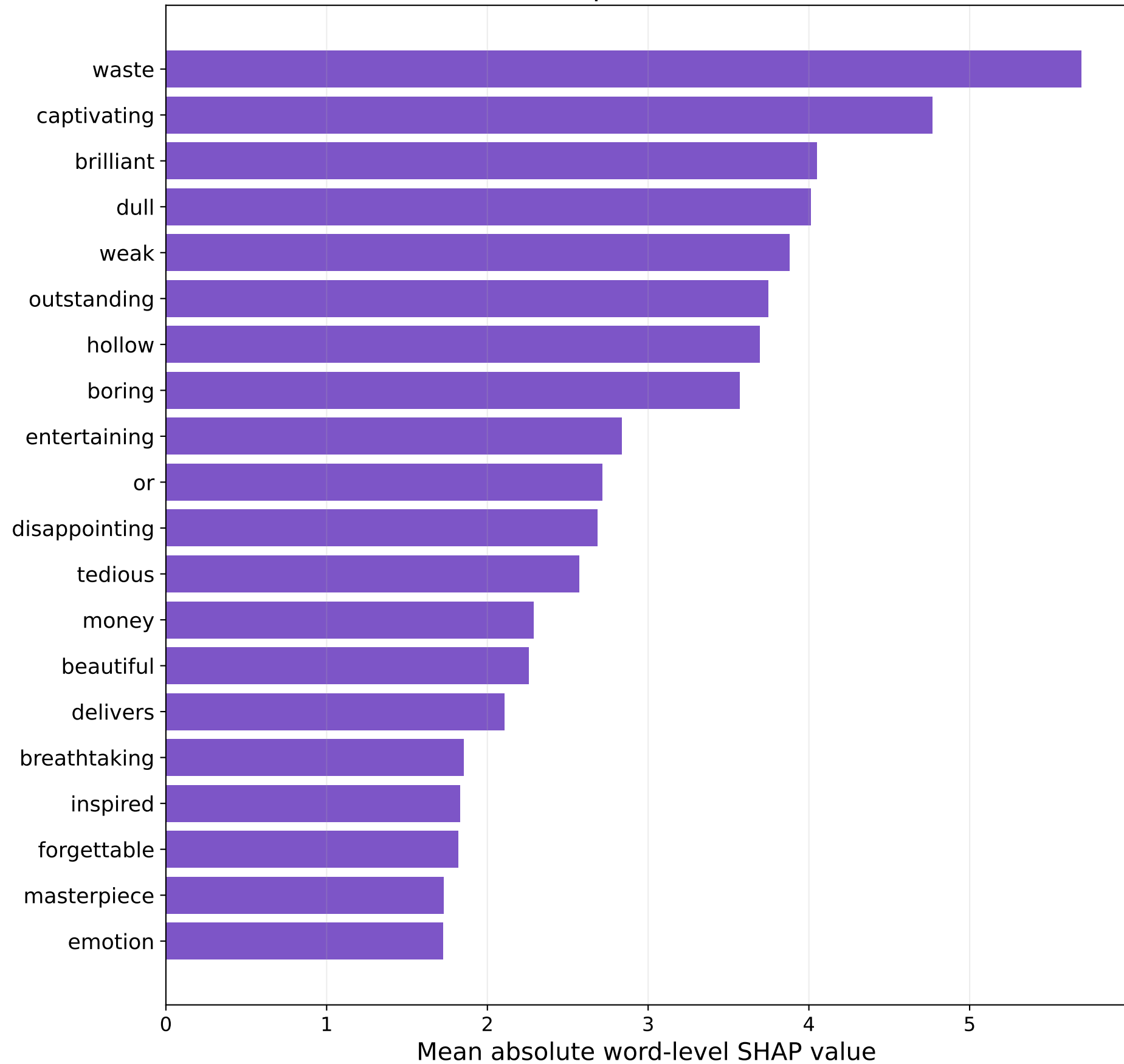
BERT SST-2 - Global comparison over selected sentences
