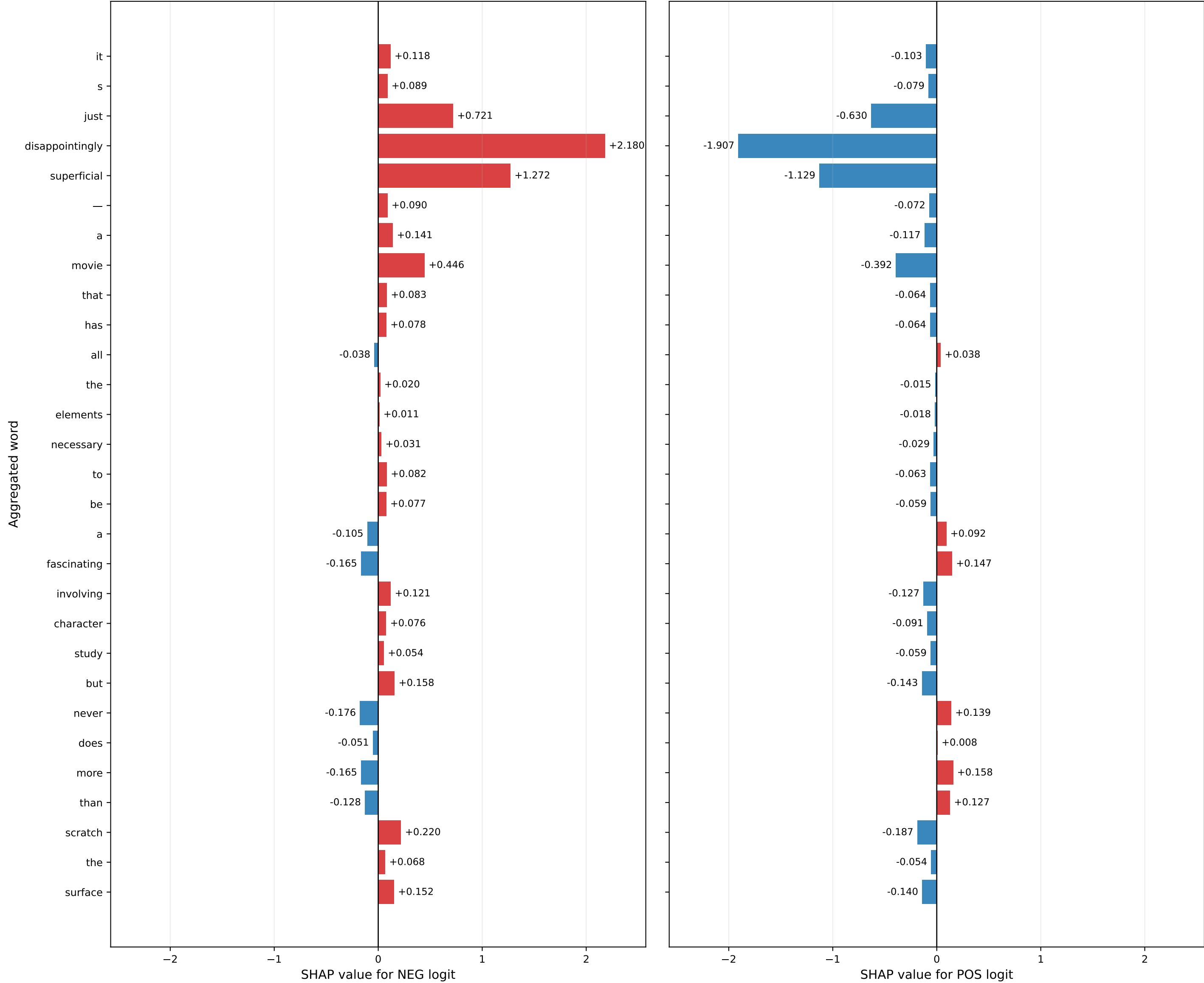
Target: NEG logit=+3.4692 | base=-2.1157 | residual=1.78e-15
