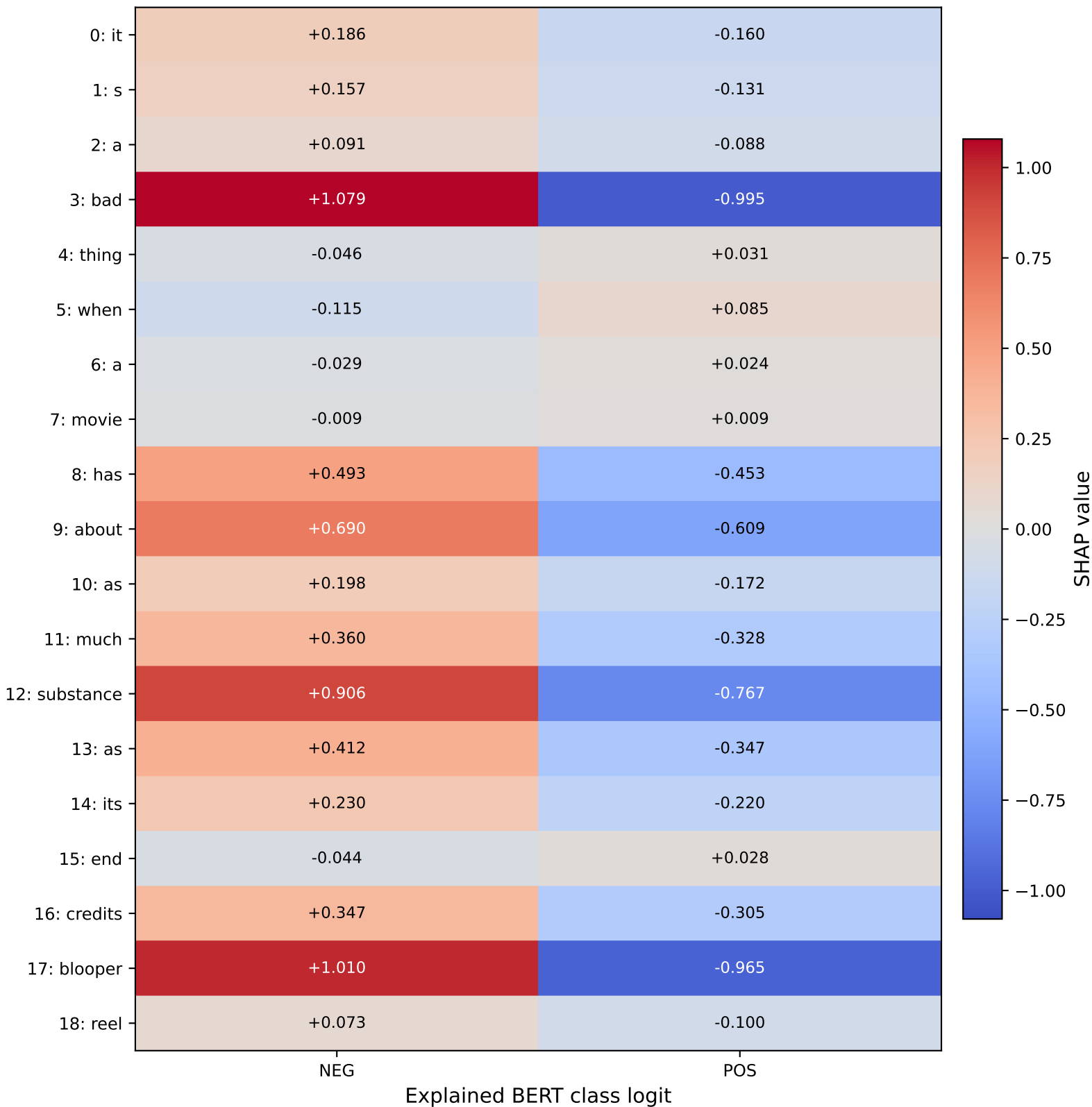
D03: Word-by-class SHAP matrix
