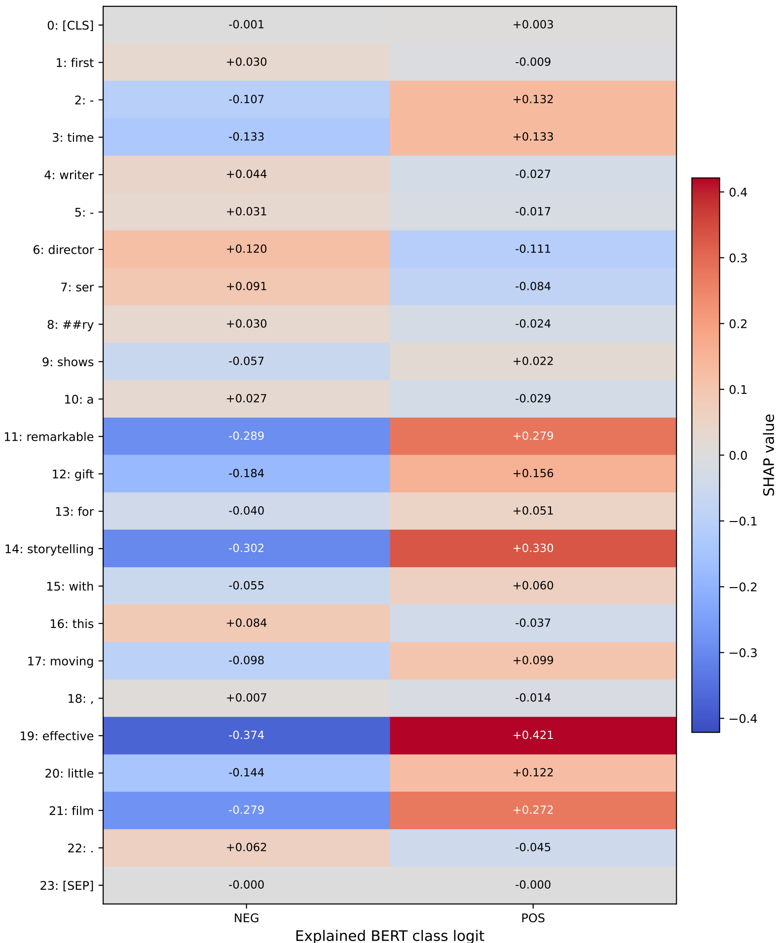
D04: Token-by-class SHAP matrix
