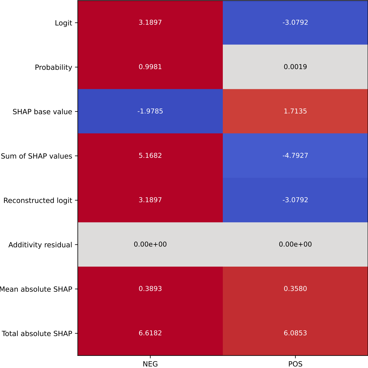
Sentence-summary values
