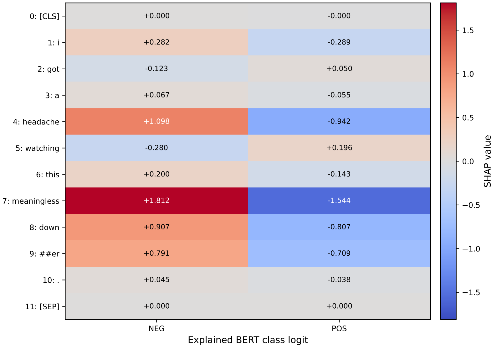
D09: Token-by-class SHAP matrix
