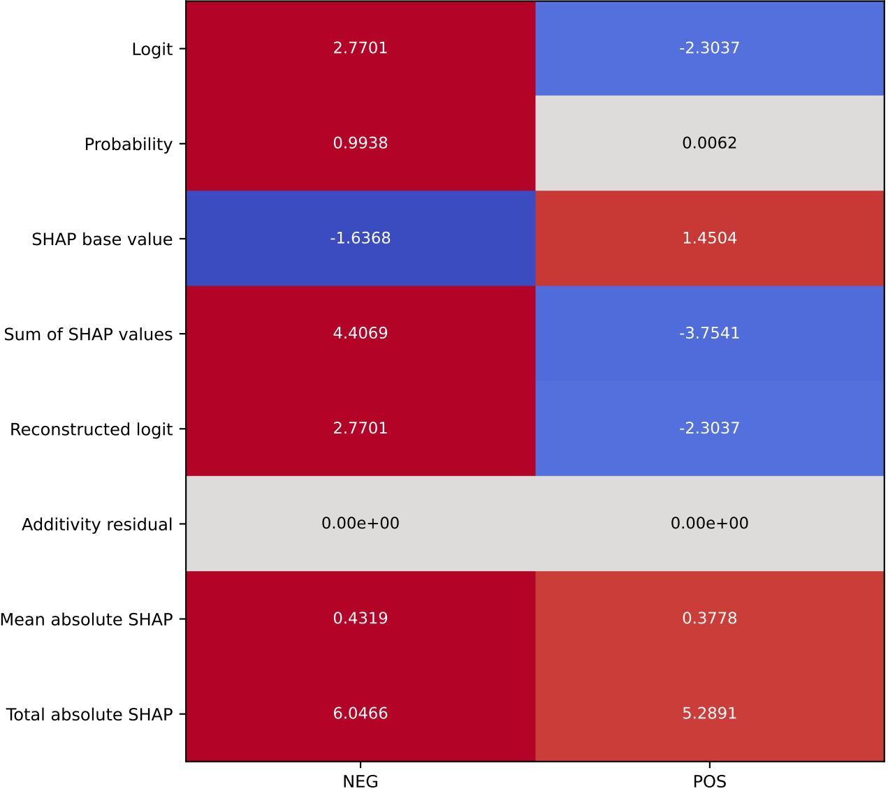
Sentence-summary values
