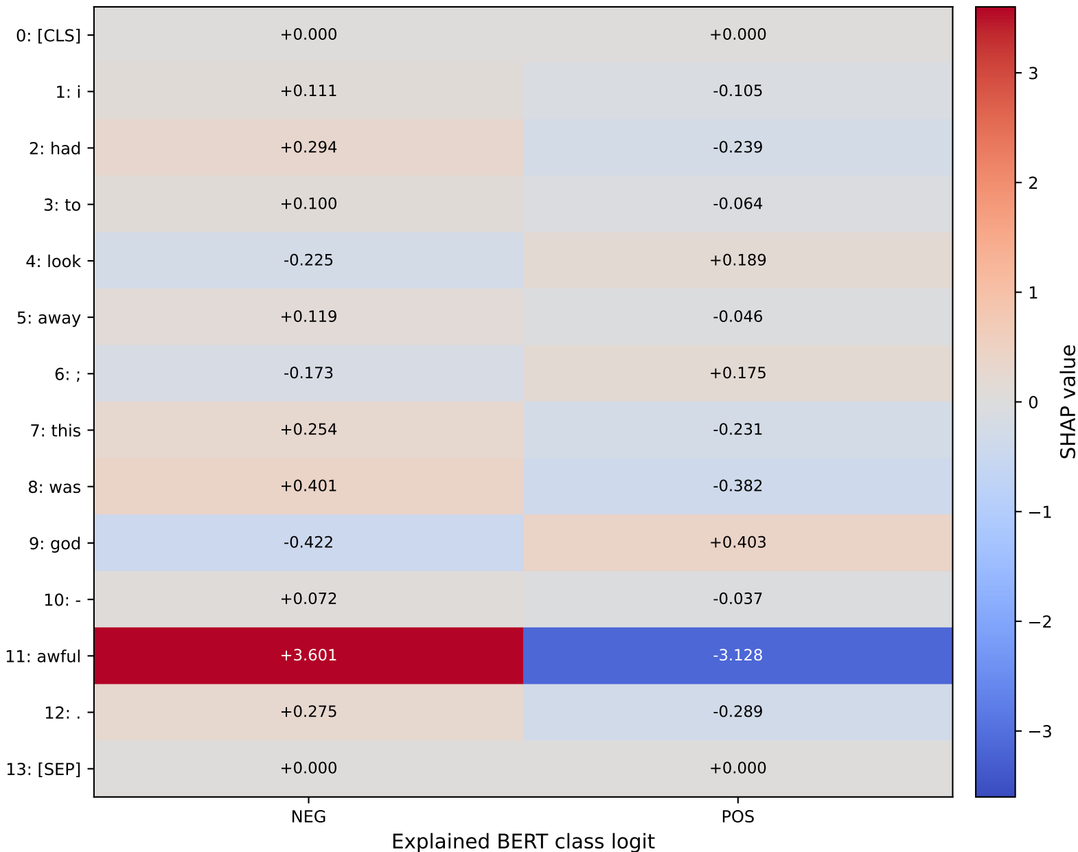
D10: Token-by-class SHAP matrix
