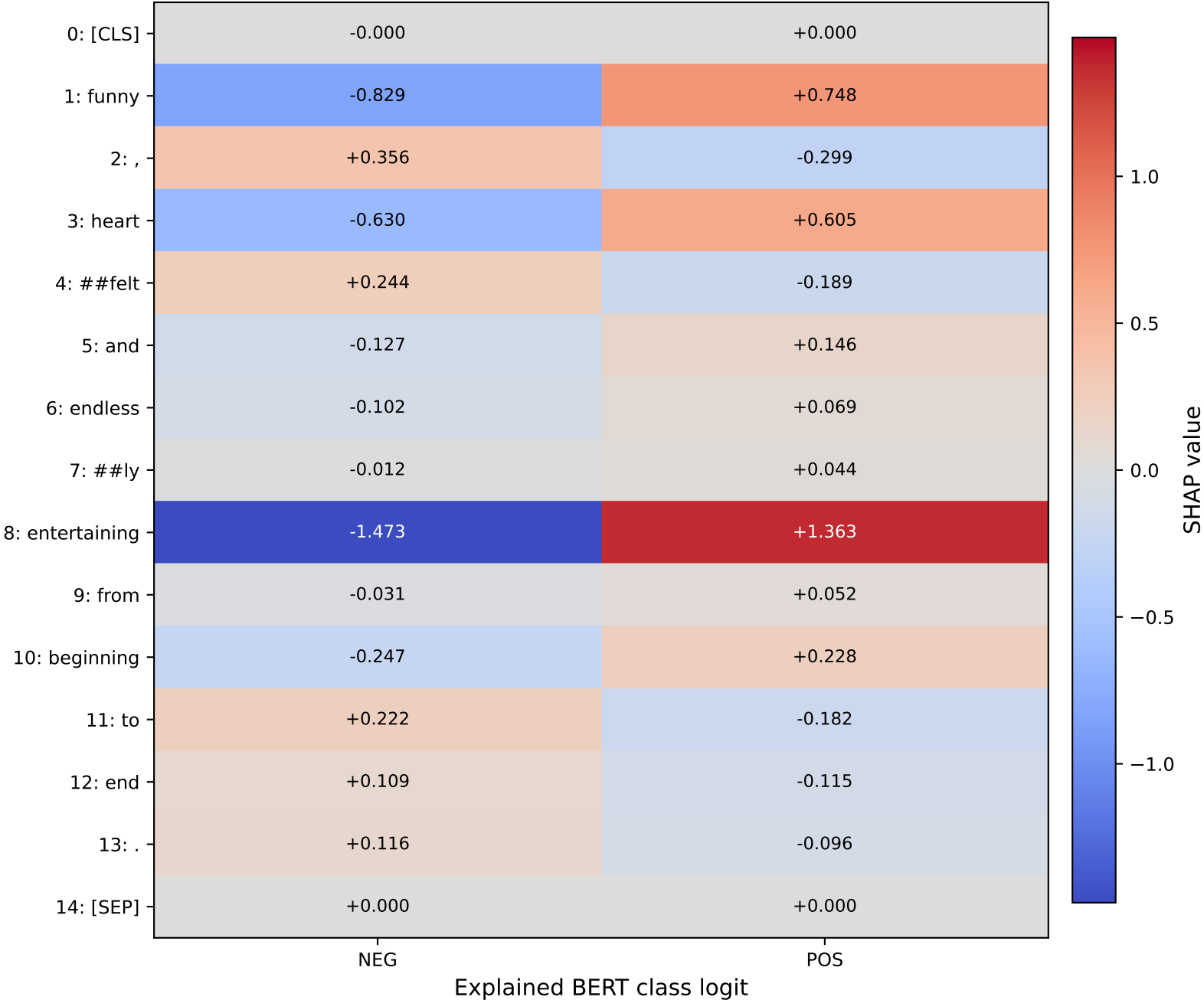
S10: Token-by-class SHAP matrix
