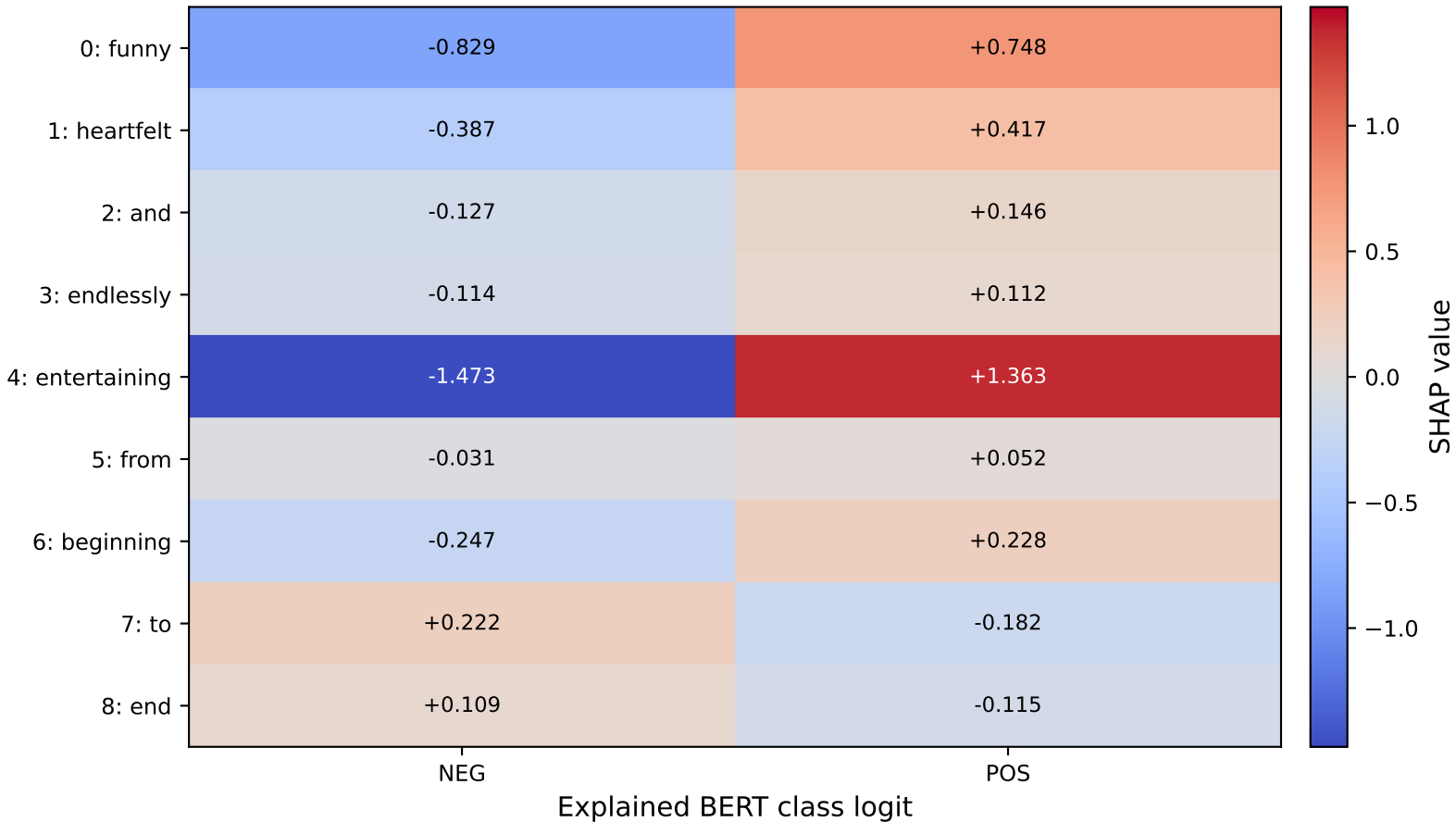
S10: Word-by-class SHAP matrix
