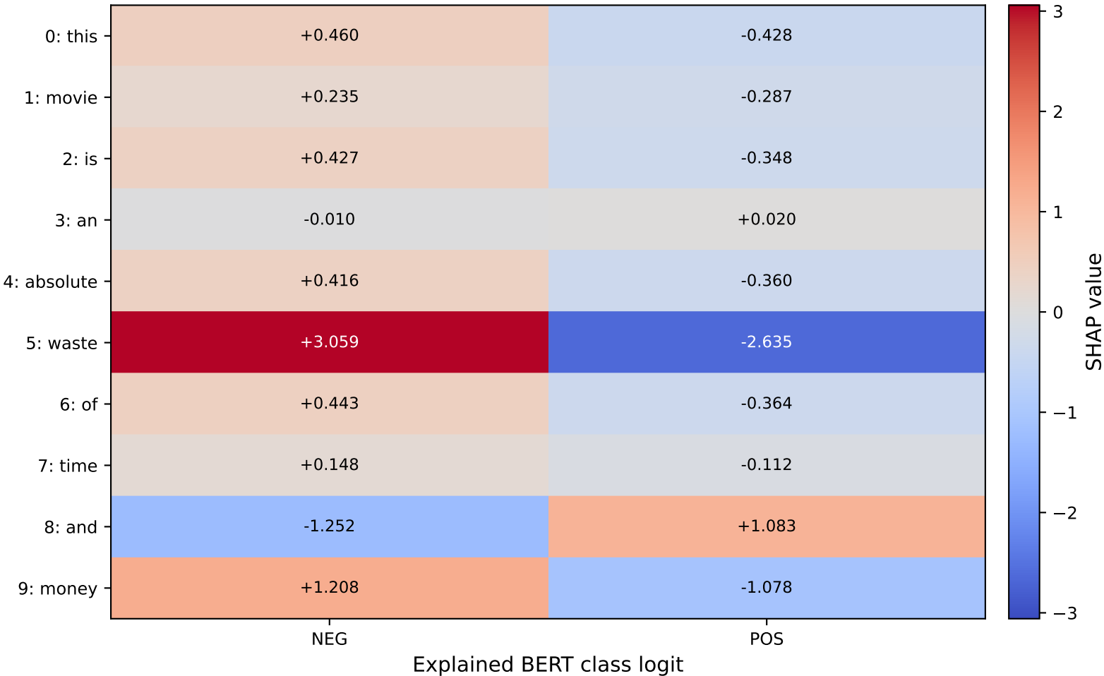
S2: Word-by-class SHAP matrix
