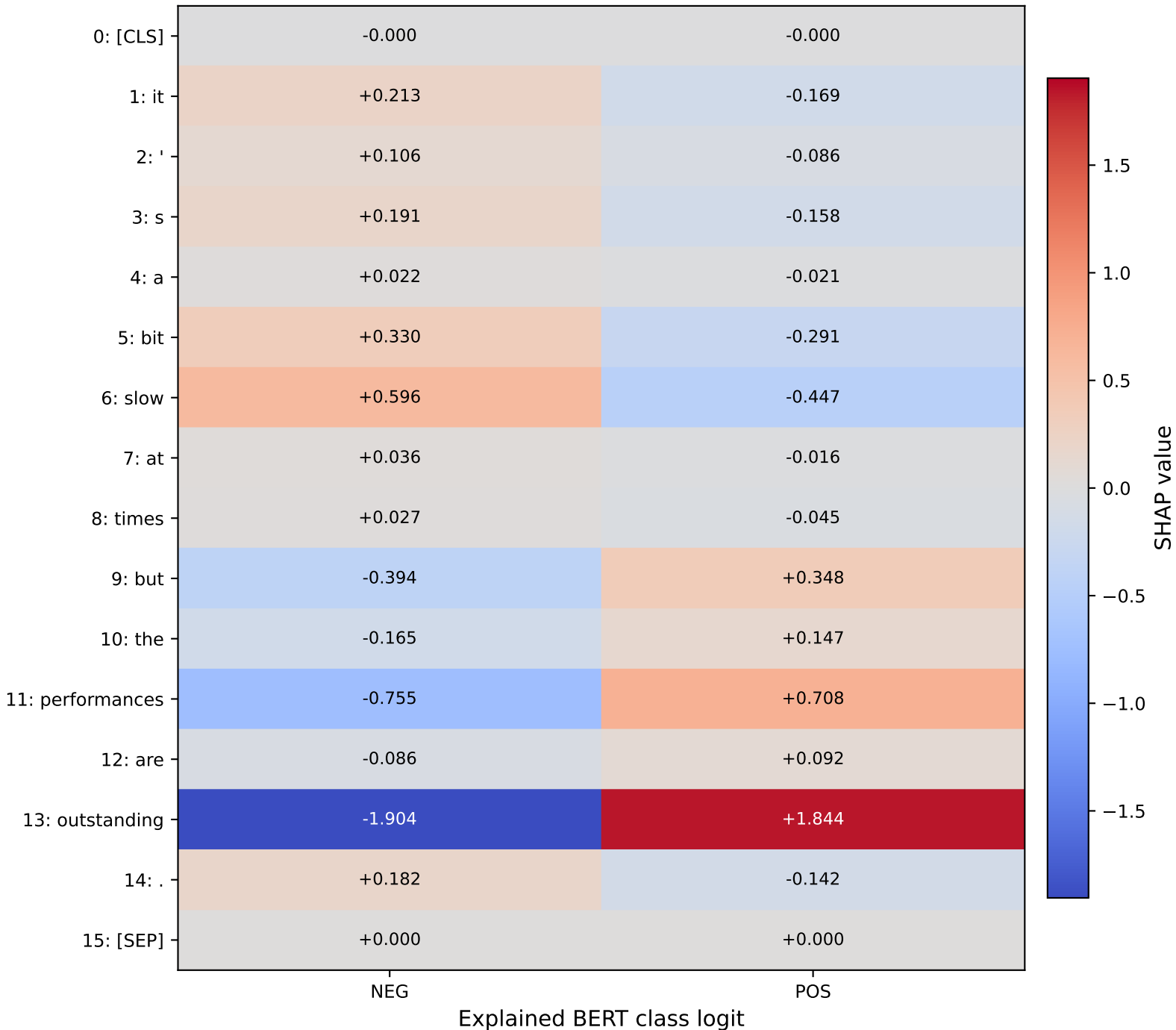
S3: Token-by-class SHAP matrix
