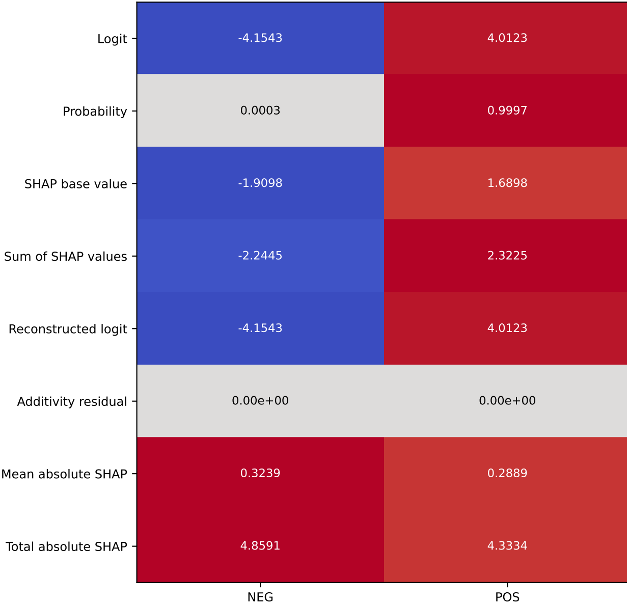
Sentence-summary values
