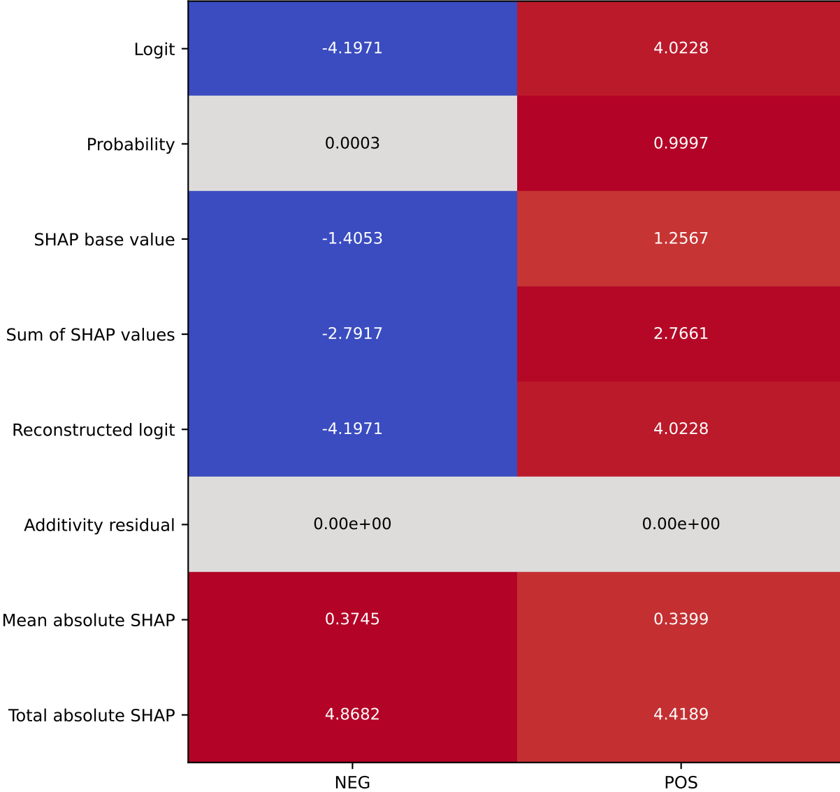
Sentence-summary values
