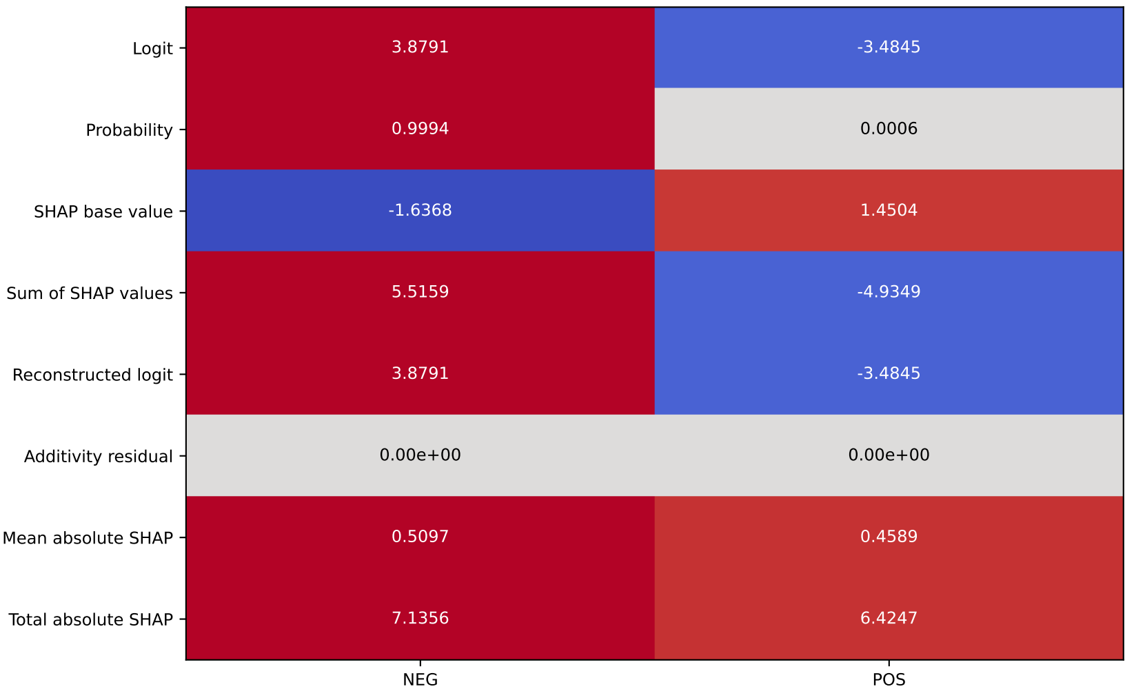
S7: sentence-summary value matrix
