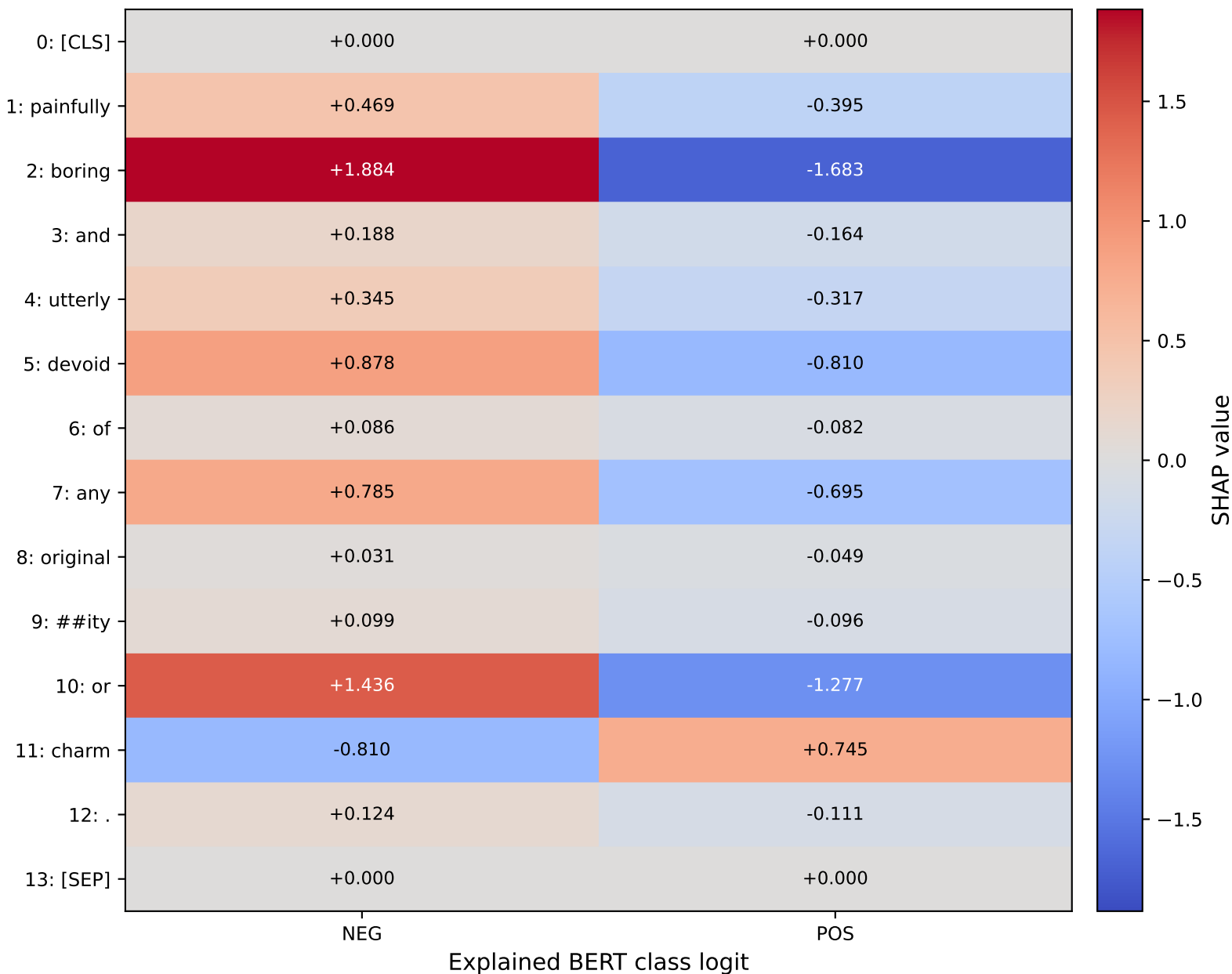
S7: Token-by-class SHAP matrix
