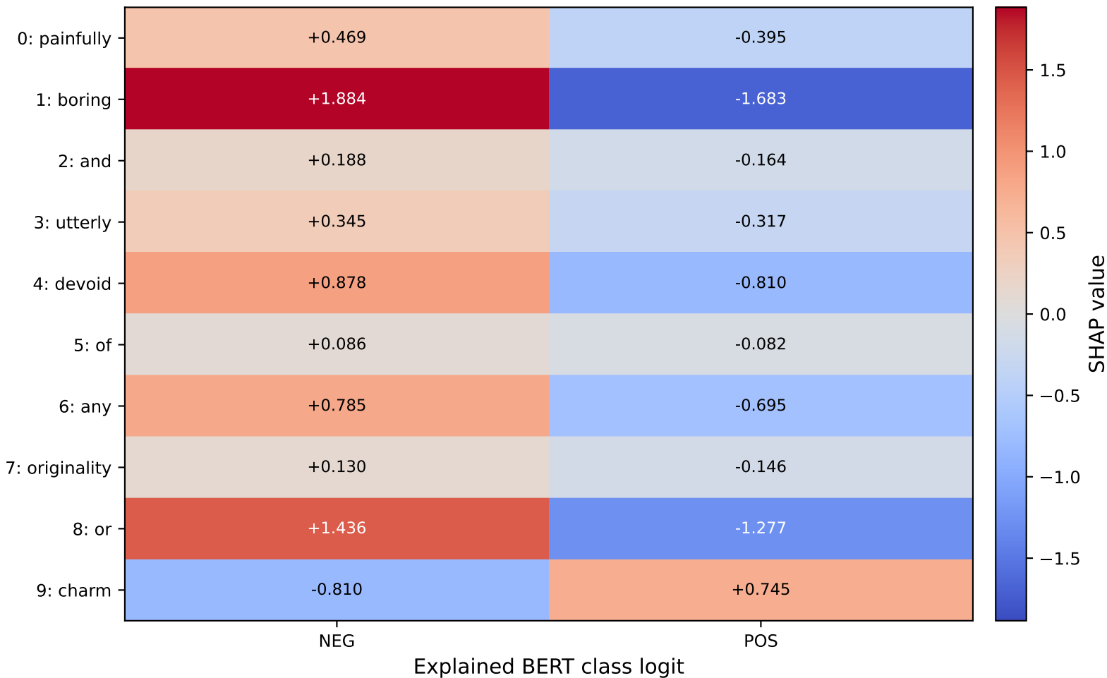
S7: Word-by-class SHAP matrix
