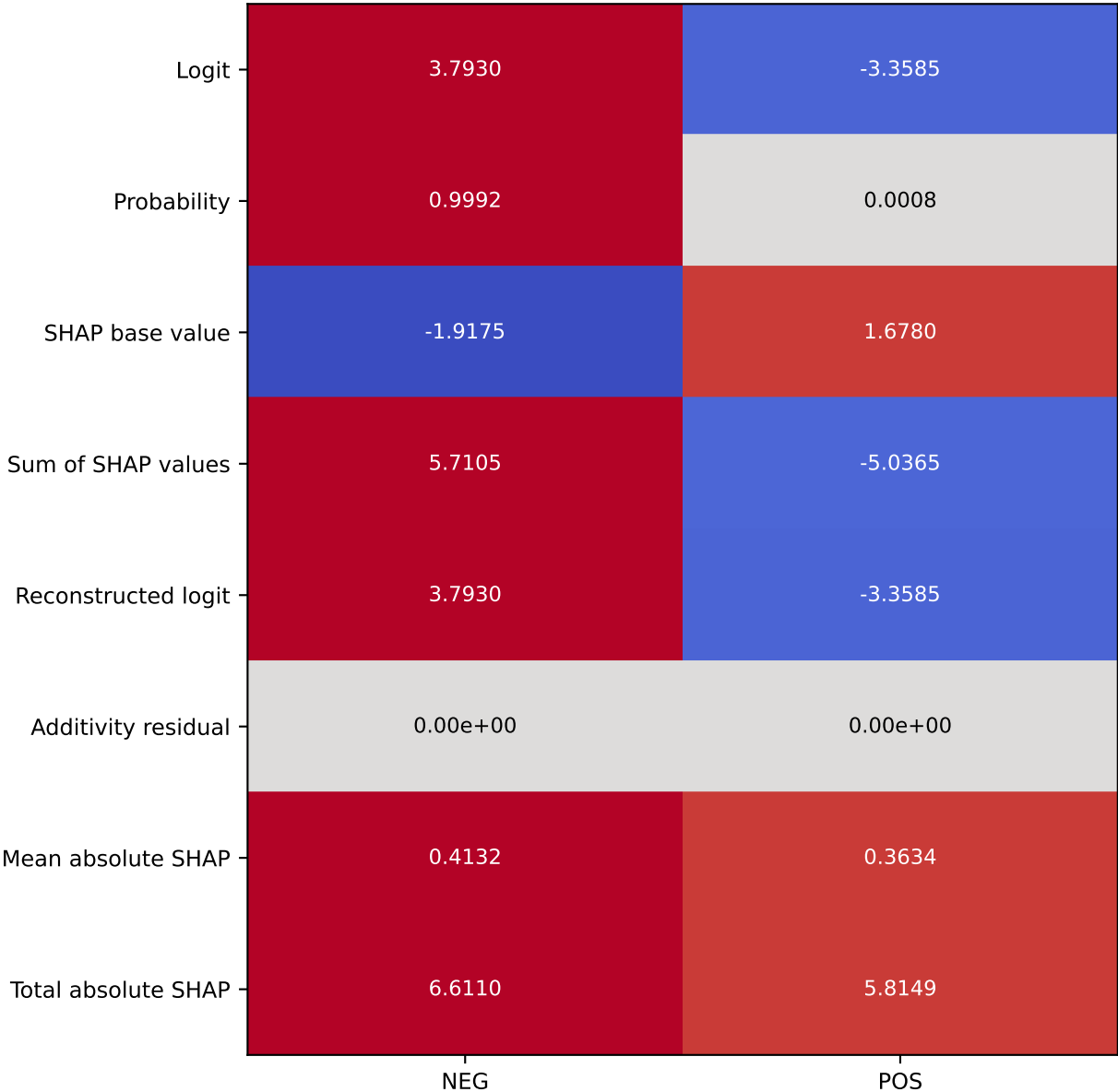
Sentence-summary values
