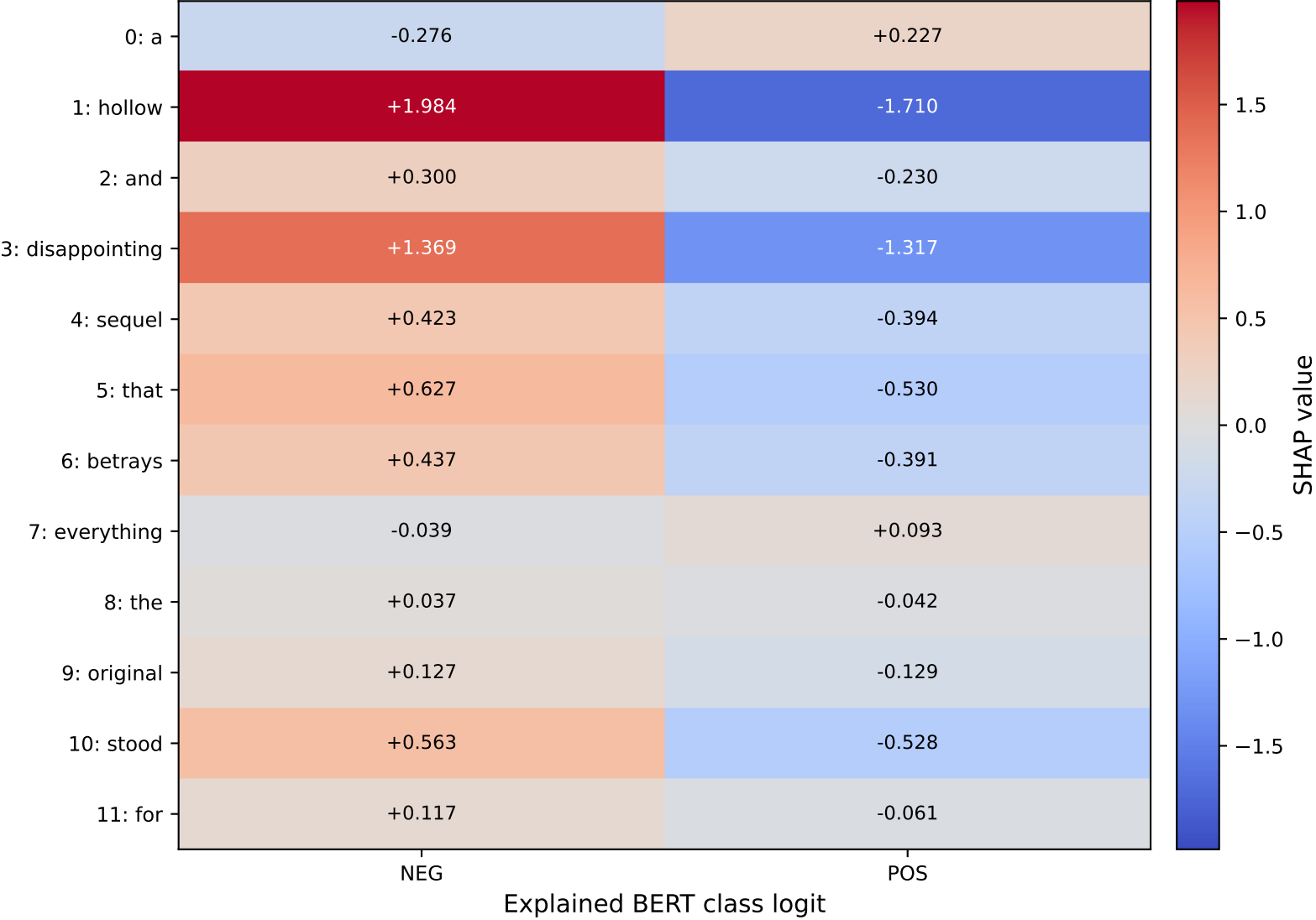
S9: Word-by-class SHAP matrix
