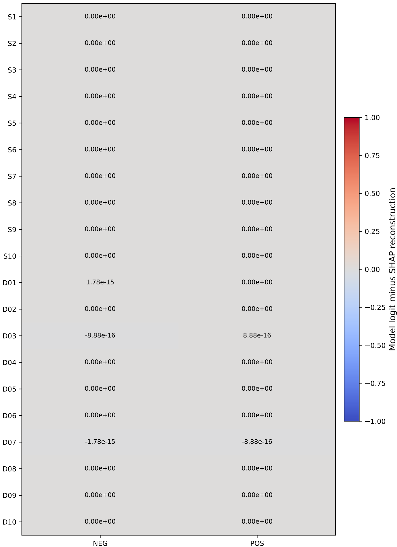
Class-specific SHAP additivity residuals
