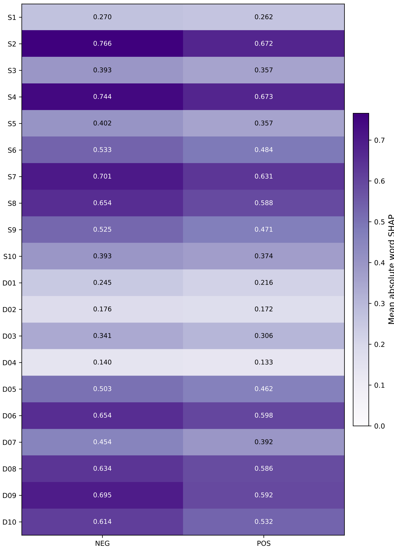
Mean absolute word-level SHAP by sentence and class
