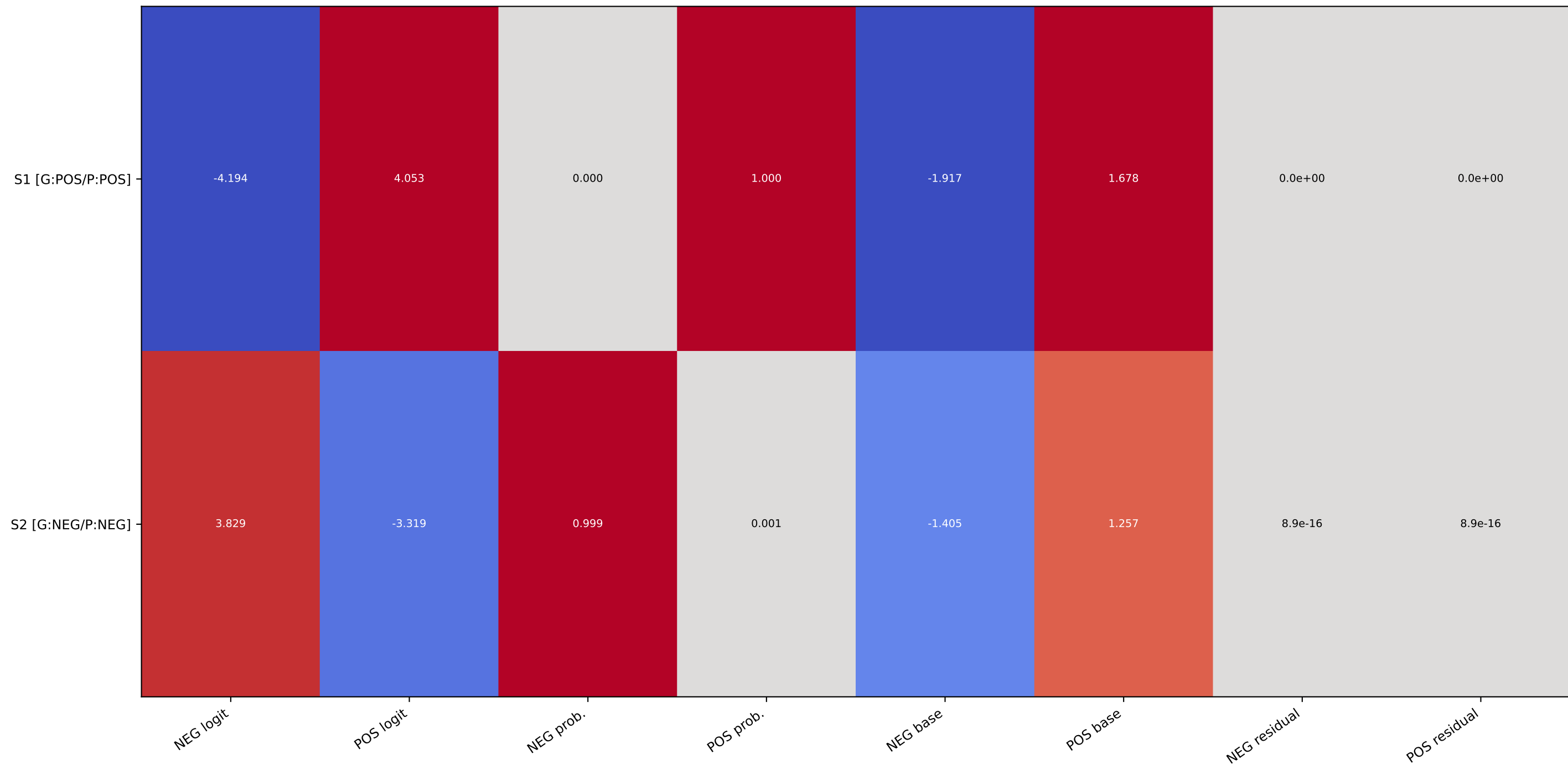
All-sentence BERT dual-class summary matrix
