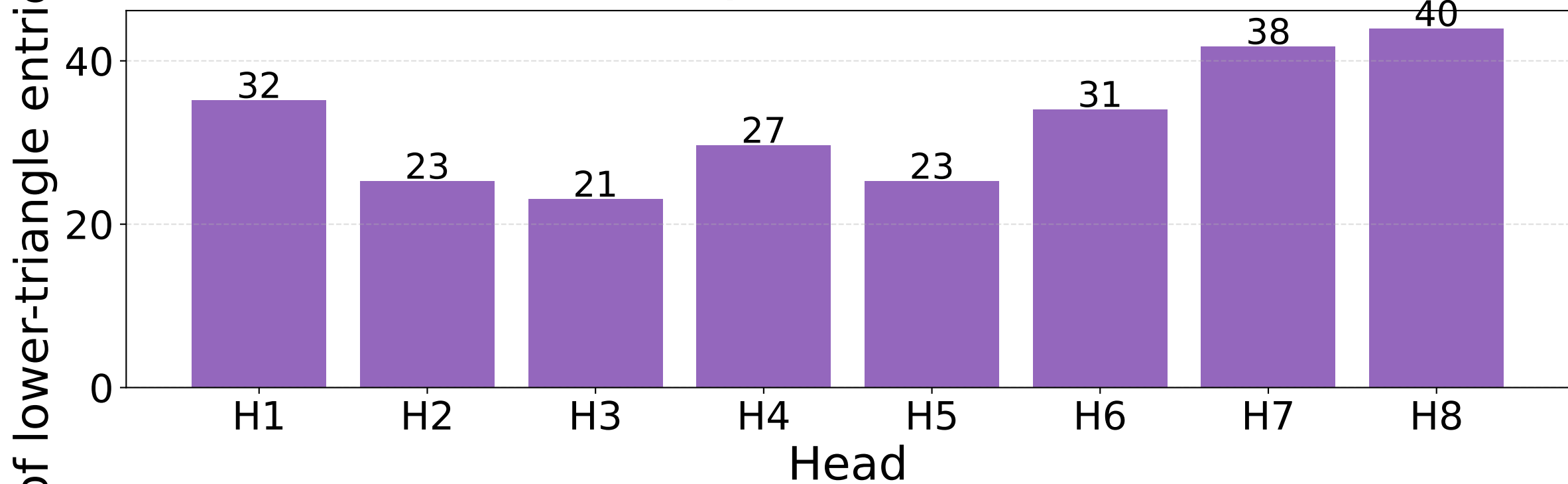
Step 2 — Mask sparsity per head (K=1.0, lower-tri only)
