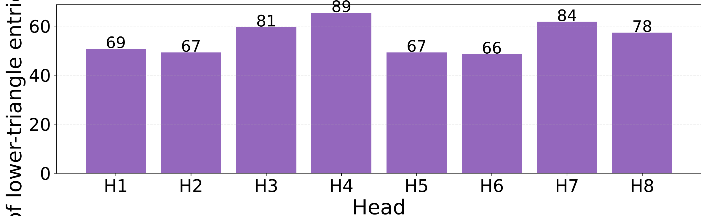
87 Step 2 — Mask sparsity per head (K=0.0, lower-tri only)
