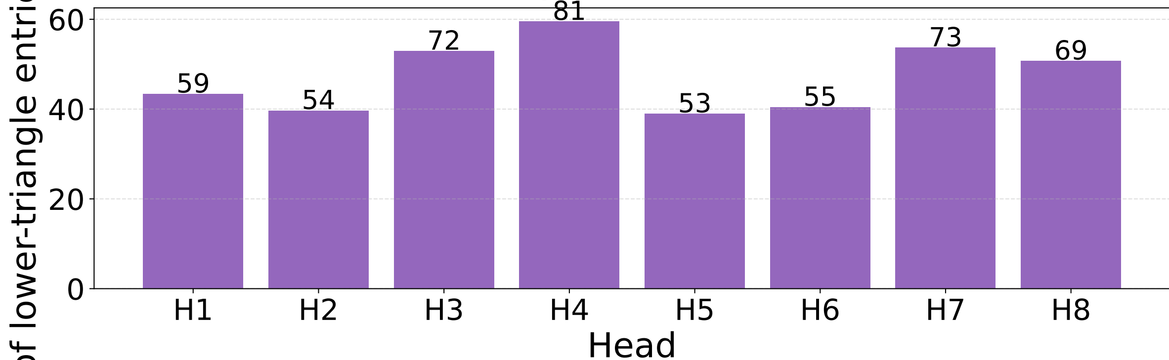
Step 2 — Mask sparsity per head (K=0.3, lower-tri only)
