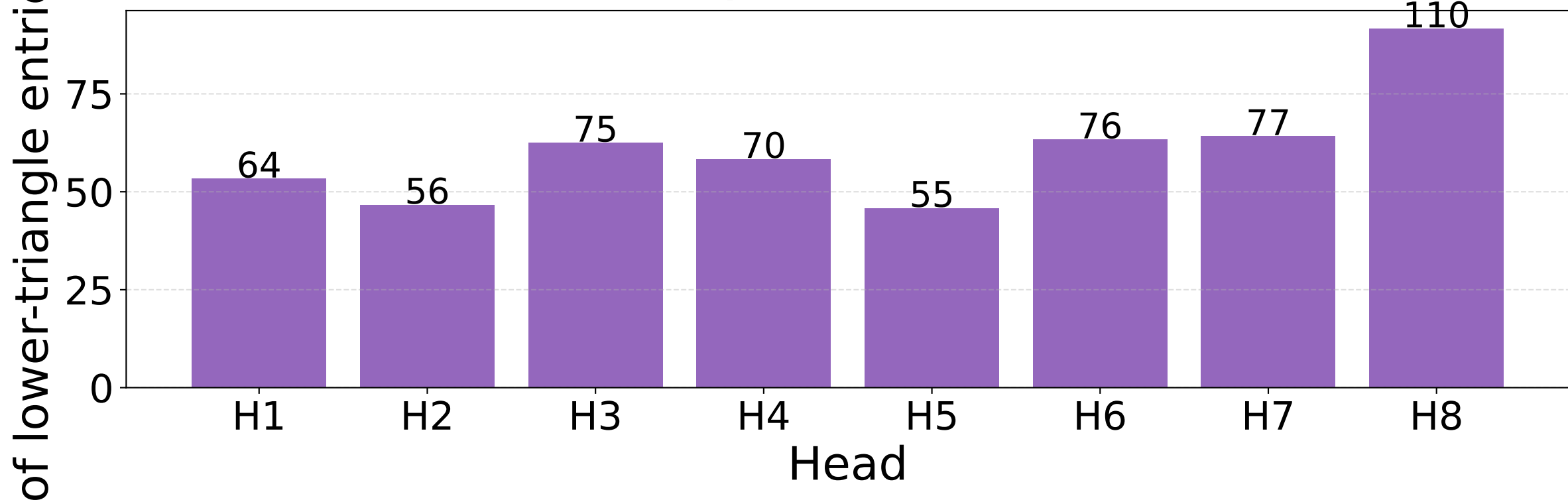
8 Step 2 — Mask sparsity per head (K=0.0, lower-tri only)
