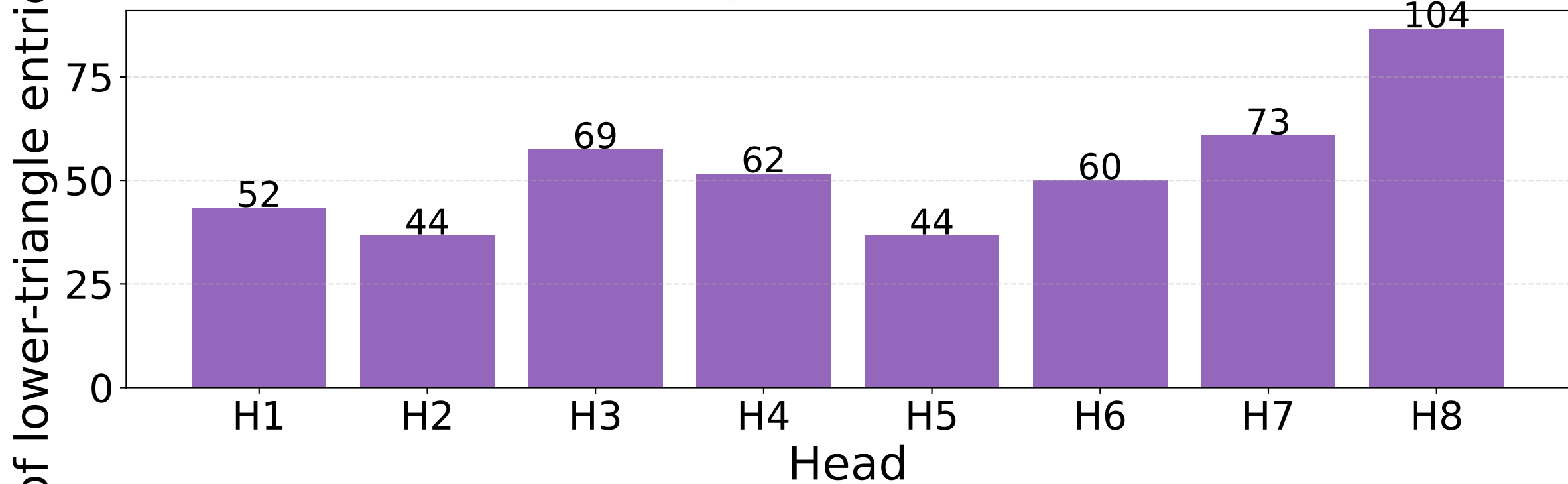
8 Step 2 — Mask sparsity per head (K=0.3, lower-tri only)
