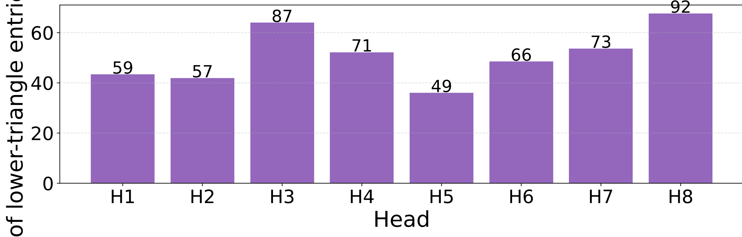
99 Step 2 — Mask sparsity per head (K=0.3, lower-tri only)
