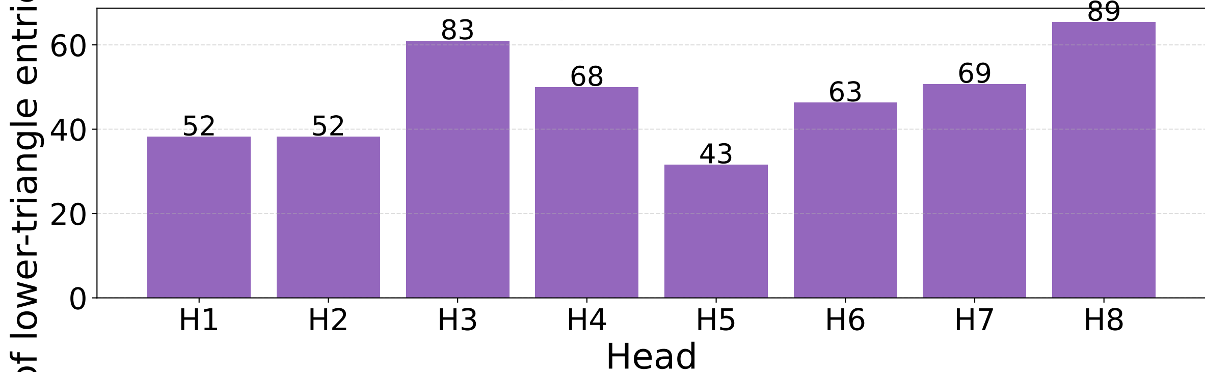
99 Step 2 — Mask sparsity per head (K=0.5, lower-tri only)
